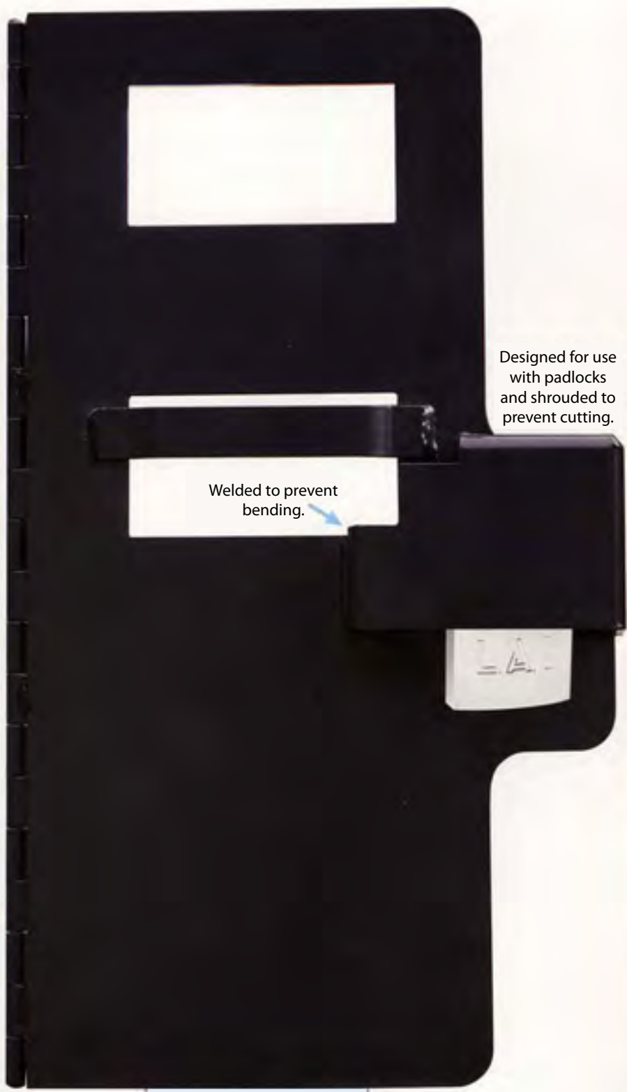
S819X Full Metal Jacket Ultimate Double Door Bar (Shown with optional B645B Padlock featured in the LAI 600 Series Catalog.)
