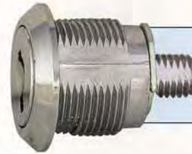
Z418D-AI-D2 - 5/8" - (18mm) Economy Camlock - Available Keyed Alike or Keyed Different - Side View Comes with Standard Tail Piece.
